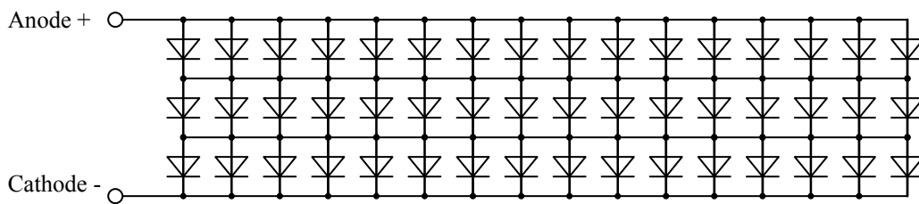
Equivalent circuit
