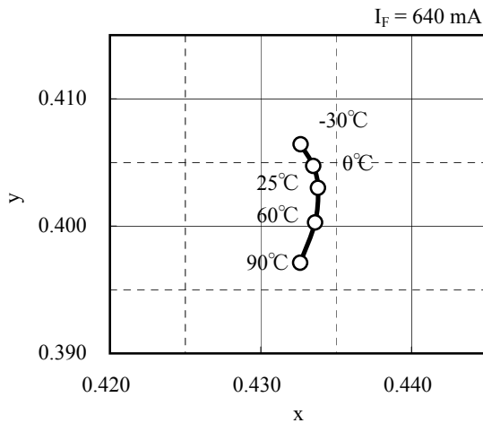
Chromaticity Coordinate vs. Case Temperature
